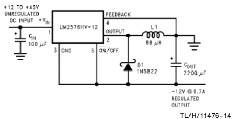
FIGURE 10. Inverting Buck-Boost Develops -12V
