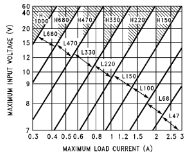
FIGURE 4. LM2576(HV)-5.0
